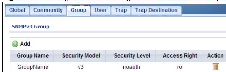
Figure 196 Configuration > Management > SNMP > Group
