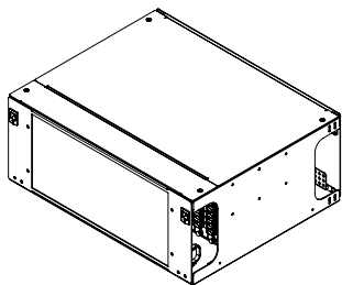
(01) L-Series AM-4RU Sliding Patch Panel
